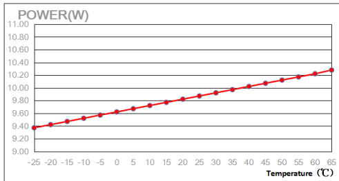
Relation of Working Temperature and Power
