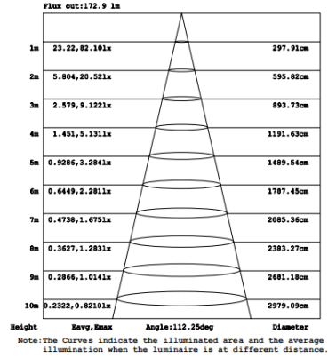
Illuminance
