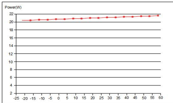
Relation of Working Temperature and Power
