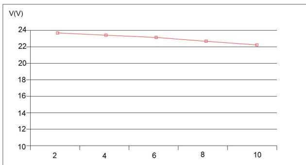
Relation of operating voltage and strip length
