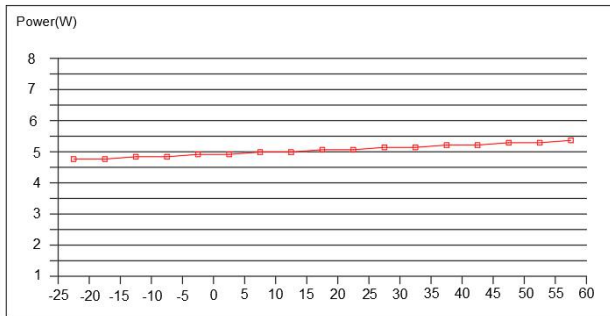
Relation of Working Temperature and Power
