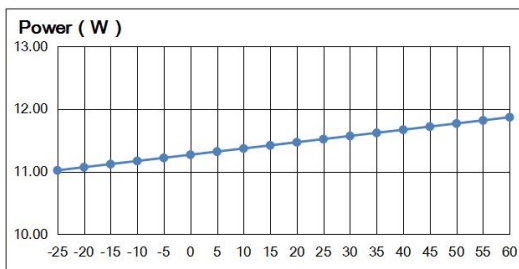
Relation of Working Temperature and Power
