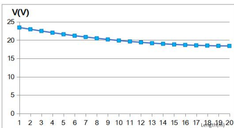
Relation of operating voltage and strip length
