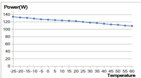
Relation of Working Temperature and Power
